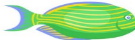
Lined surgeonfish
